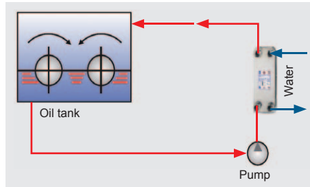
Oil cooling
