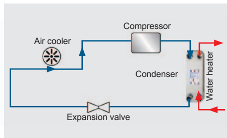
Heat pump
