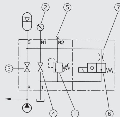
Circuit diagram
